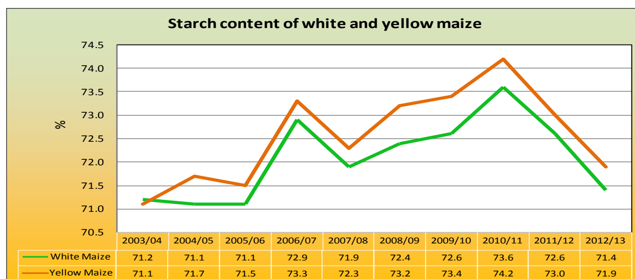
Graph 39: Starch content of white and yellow maize over 10 seasons
